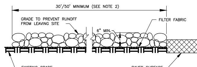
PROFILE VIEW
