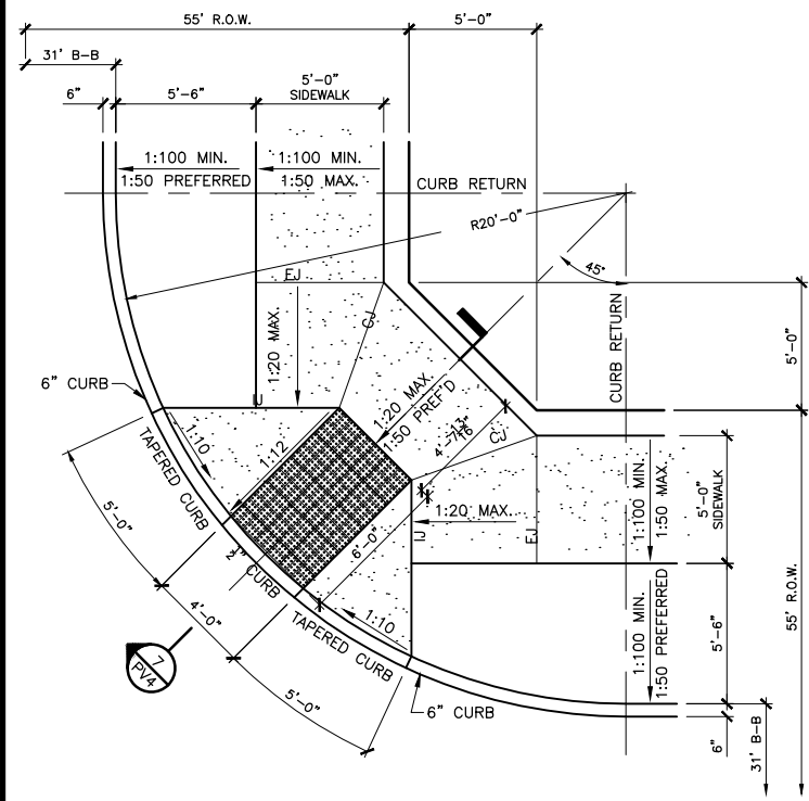
31-FOOT BACK-TO-BACK OF CURB STREET WIDTH
