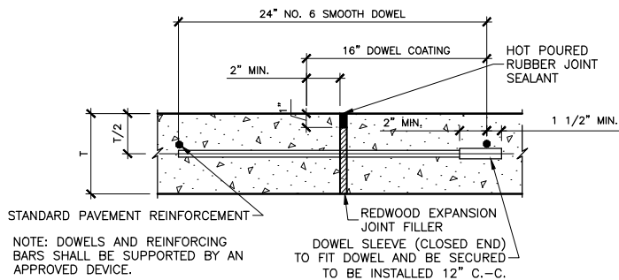
⑤ TRANSVERSE EXPANSION JOINT NO SCALE
