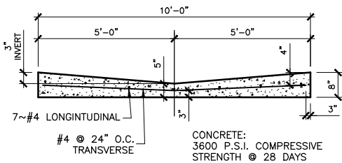
① TYPICAL 10' ALLEY SECTION NO SCALE
