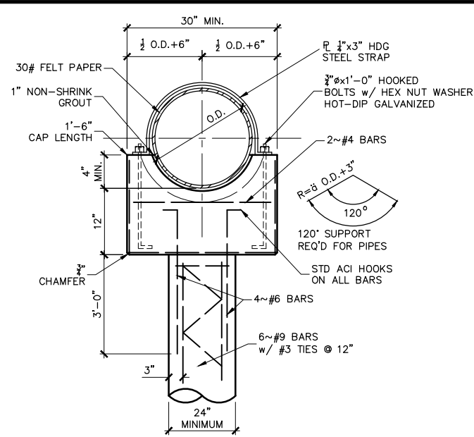
2 AERIAL CROSSING PIER CAP DETAIL NO SCALE
