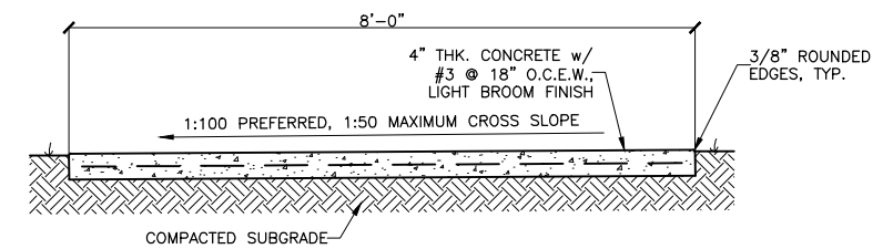
⑤ BIKE PATH SECTION 3/4"=1'-0"
