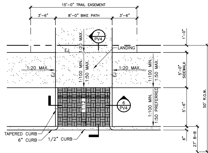
27-FOOT BACK-TO-BACK OF CURB STREET WIDTH
