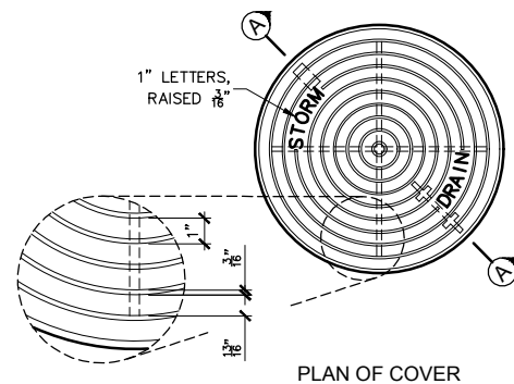
6 PLAN OF COVER NO SCALE
