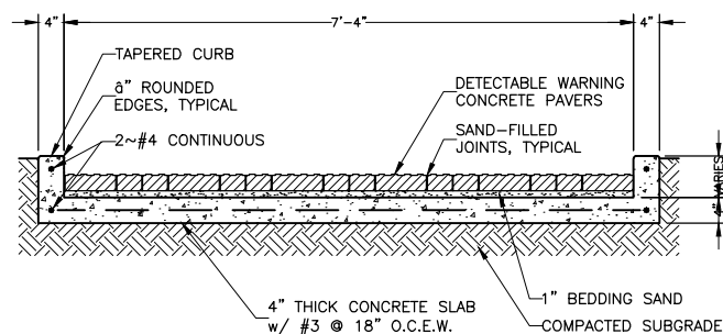
⑥ RAMP SECTION 3/4"=1'-0"
