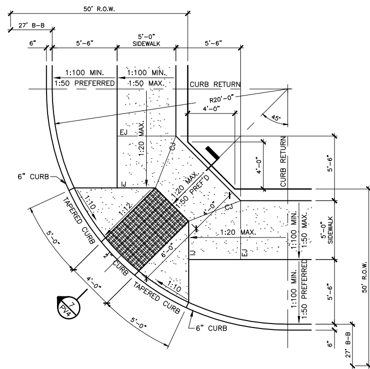
27-FOOT BACK-TO-BACK OF CURB STREET WIDTH
