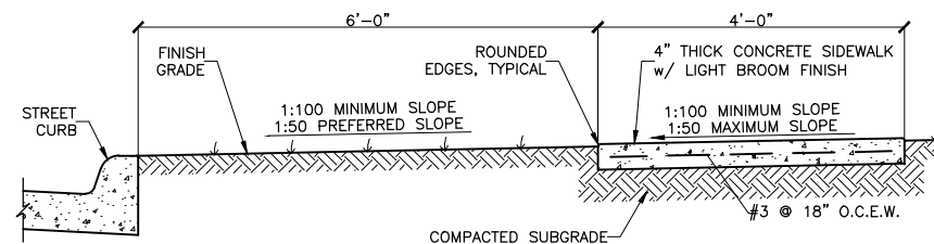
④ SIDEWALK SECTION - RESIDENTIAL ZONE 3/4"=1'-0"
