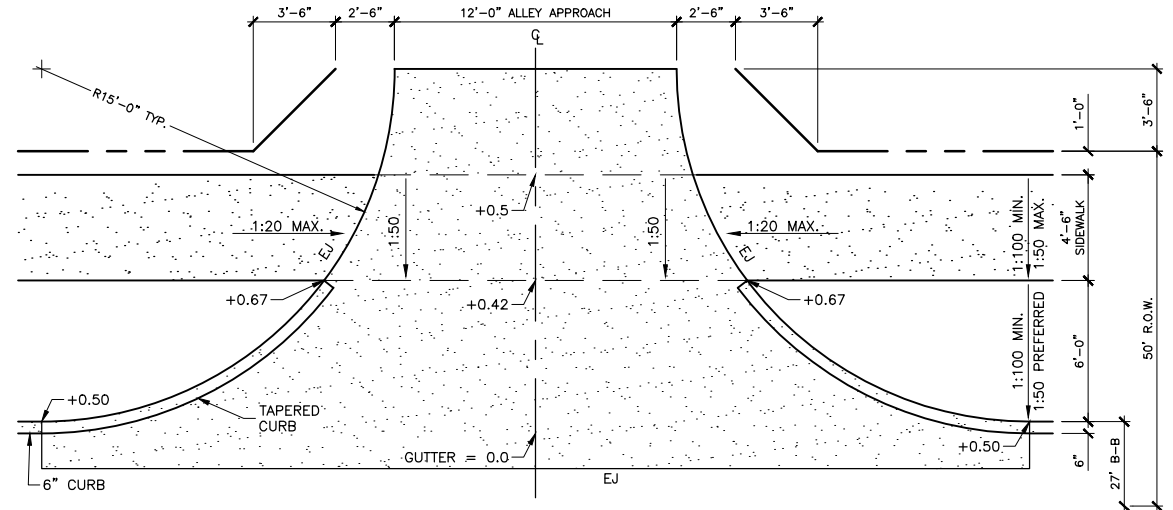
27-FOOT BACK-TO-BACK OF CURB STREET WIDTH
