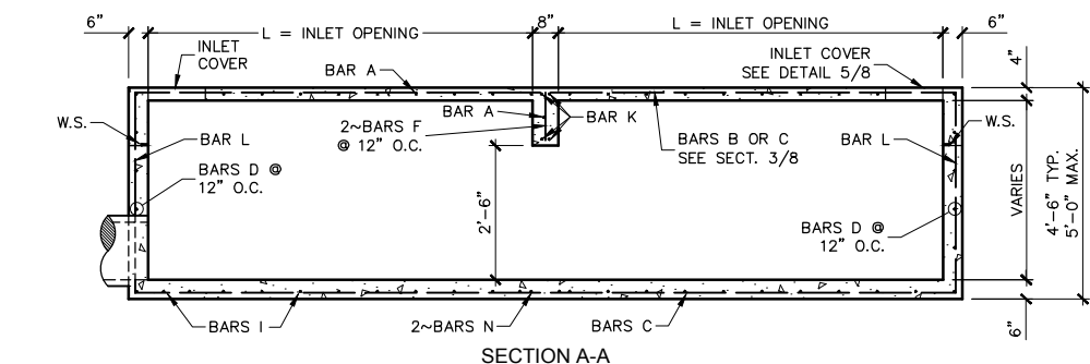
8 DOUBLE INLET DETAILS NO SCALE
