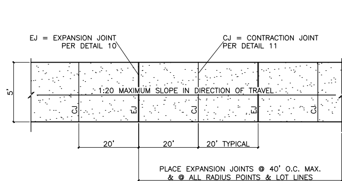
① SIDEWALK PLAN - COMMERCIAL ZONE 1/4"=1'-0"
