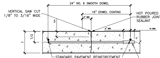
⑦ CONTRACTION JOINT NO SCALE
