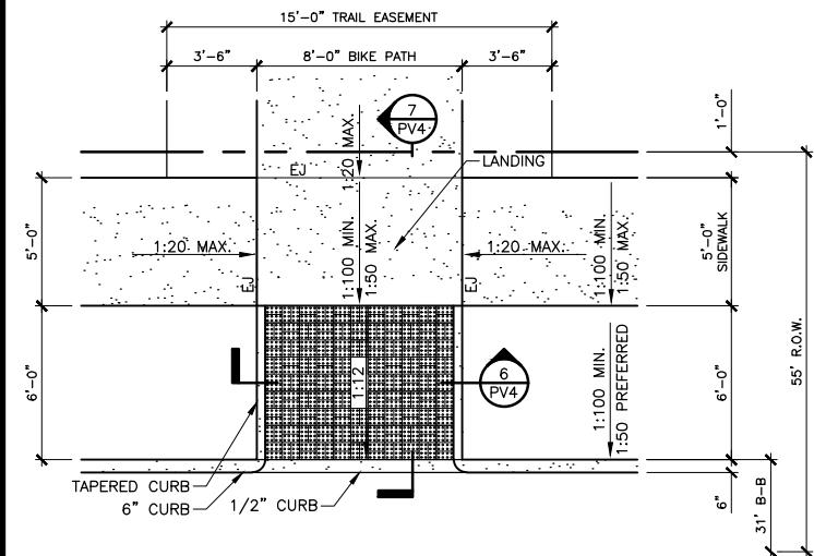
31-FOOT BACK-TO-BACK OF CURB STREET WIDTH
