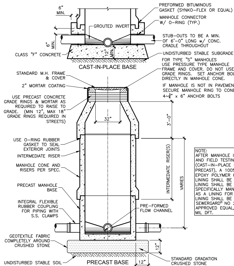
② STANDARD PRECAST MANHOLE NO SCALE
