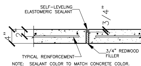
⑩ SIDEWALK EXPANSION JOINT (EJ) 1 1/2"=1'-0"
