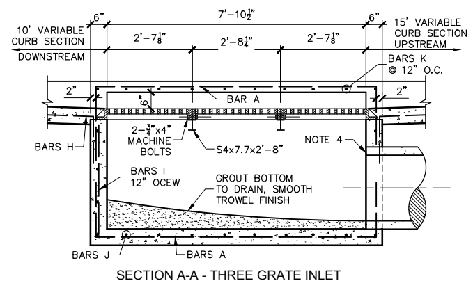
SECTION A-A - THREE GRATE INLET
