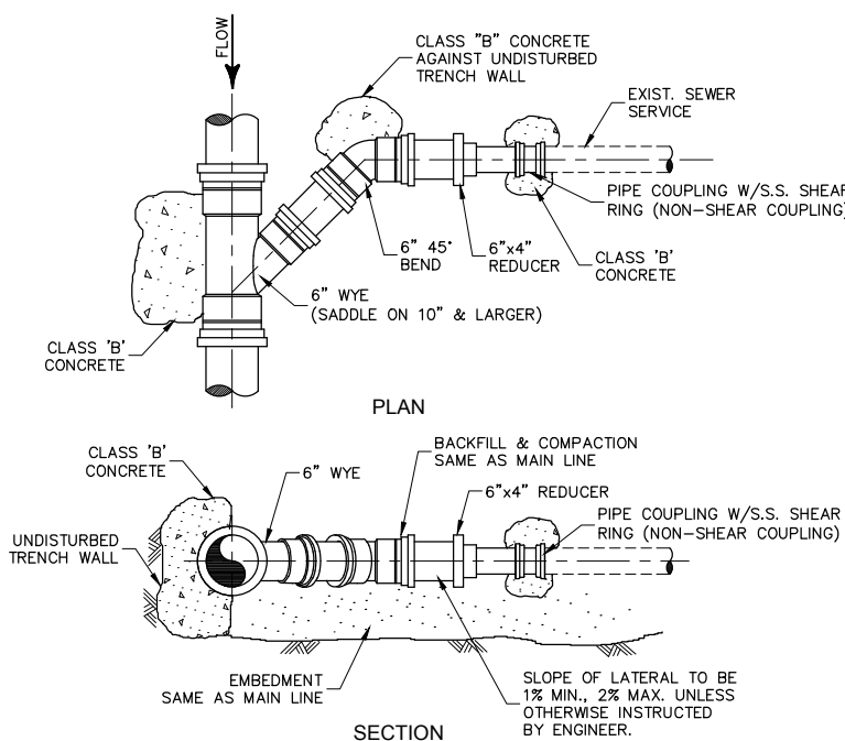
7 SANITARY SEWER SERVICE NO SCALE
