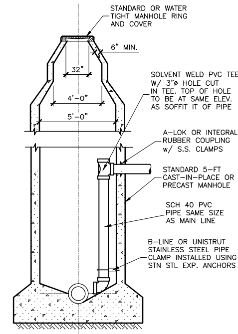
④ STANDARD 5' DROP MANHOLE CONNECTION NO SCALE
