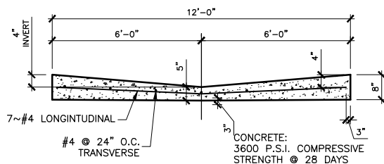
② TYPICAL 12' ALLEY SECTION NO SCALE
