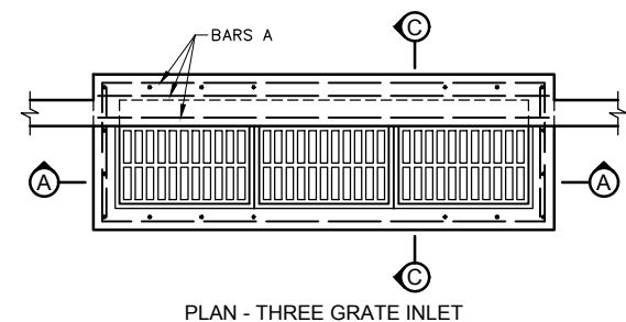
PLAN - THREE GRATE INLET
