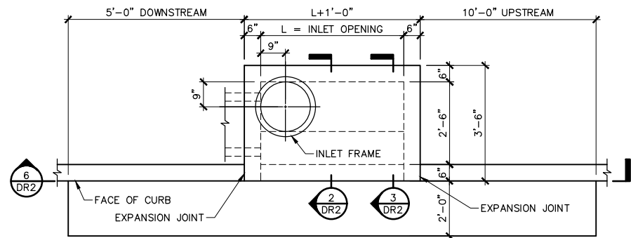
1 PLAN - STANDARD INLET NO SCALE
