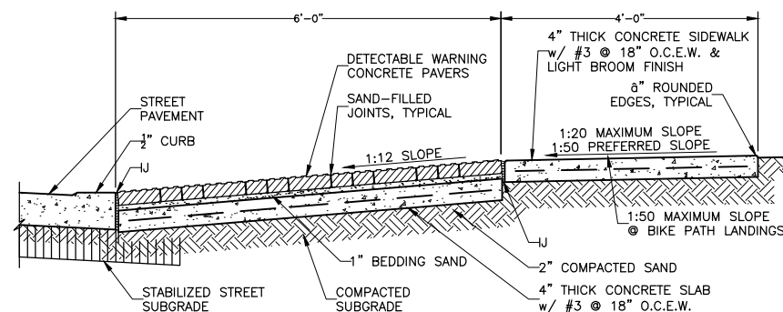
⑦ RAMP SECTION 3/4"=1'-0"
