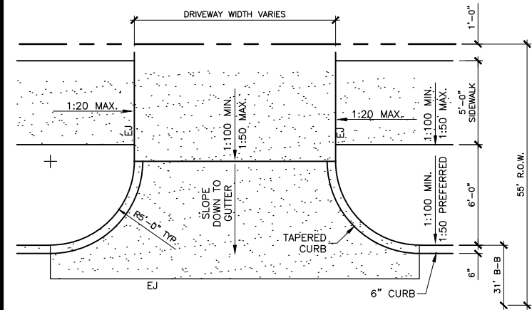
31-FOOT BACK-TO-BACK OF CURB STREET WIDTH
