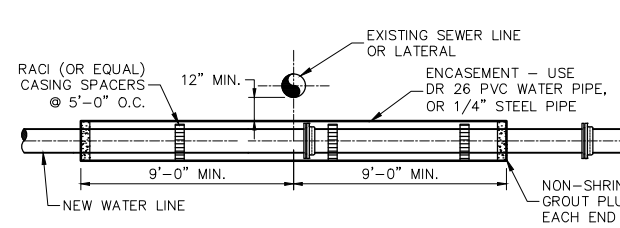
NEW WATER LINE UNDER EXISTING SEWER LINE
