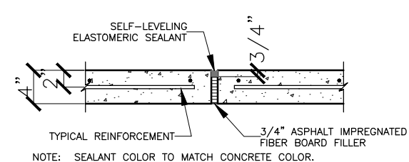
⑪ SIDEWALK ISOLATION JOINT (IJ) 1 1/2"=1'-0"
