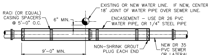
NEW SEWER LINE UNDER WATER LINE- OPTION 2
