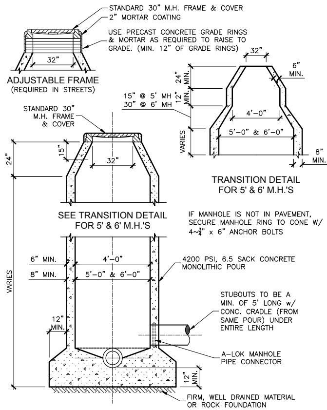
① STANDARD CAST-IN-PLACE MANHOLE NO SCALE
