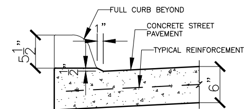
⑧ 1/2" CURB 1 1/2"=1'-0"
