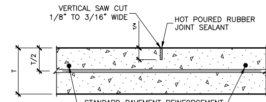
⑧ SAWED DUMMY JOINT NO SCALE
