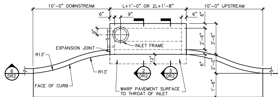
4 PLAN - RECESSED INLET NO SCALE
