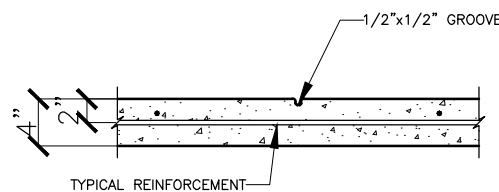
⑨ SIDEWALK CONTRACTION JOINT (CJ) 1 1/2"=1'-0"
