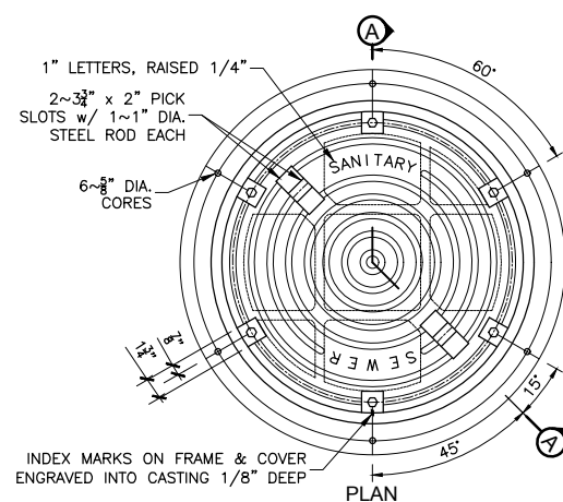
⑥ WATER TIGHT MANHOLE FRAME & COVER NO SCALE
