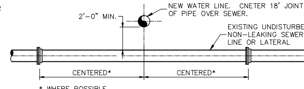
NEW WATER LINE OVER EXISTING SEWER LINE
