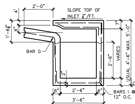
2 INLET SECTION NO SCALE
