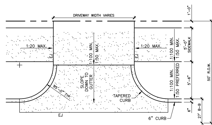
27-FOOT BACK-TO-BACK OF CURB STREET WIDTH
