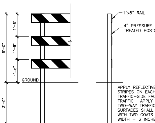
POST DETAIL
