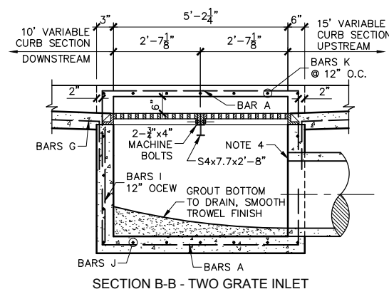
SECTION B-B - TWO GRATE INLET
