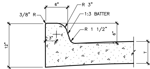
③ INTEGRAL CURB DETAIL NO SCALE
