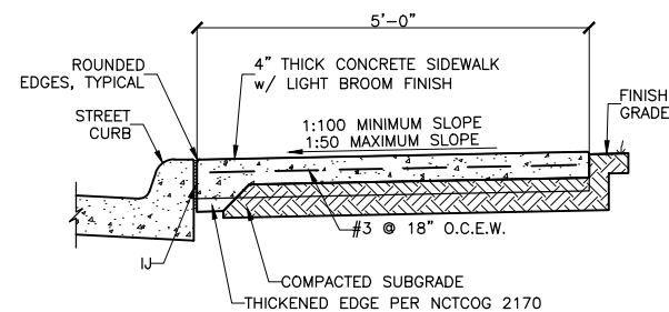
③ SIDEWALK SECTION - COMMERCIAL ZONE 3/4"=1'-0"
